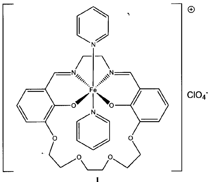
Figure 6 – Complexe 1 .
