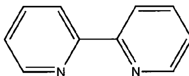
Figure 4 – 2,2-bipyridine (bipy).
