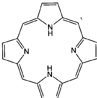
Figure 9 – Porphyrine.
